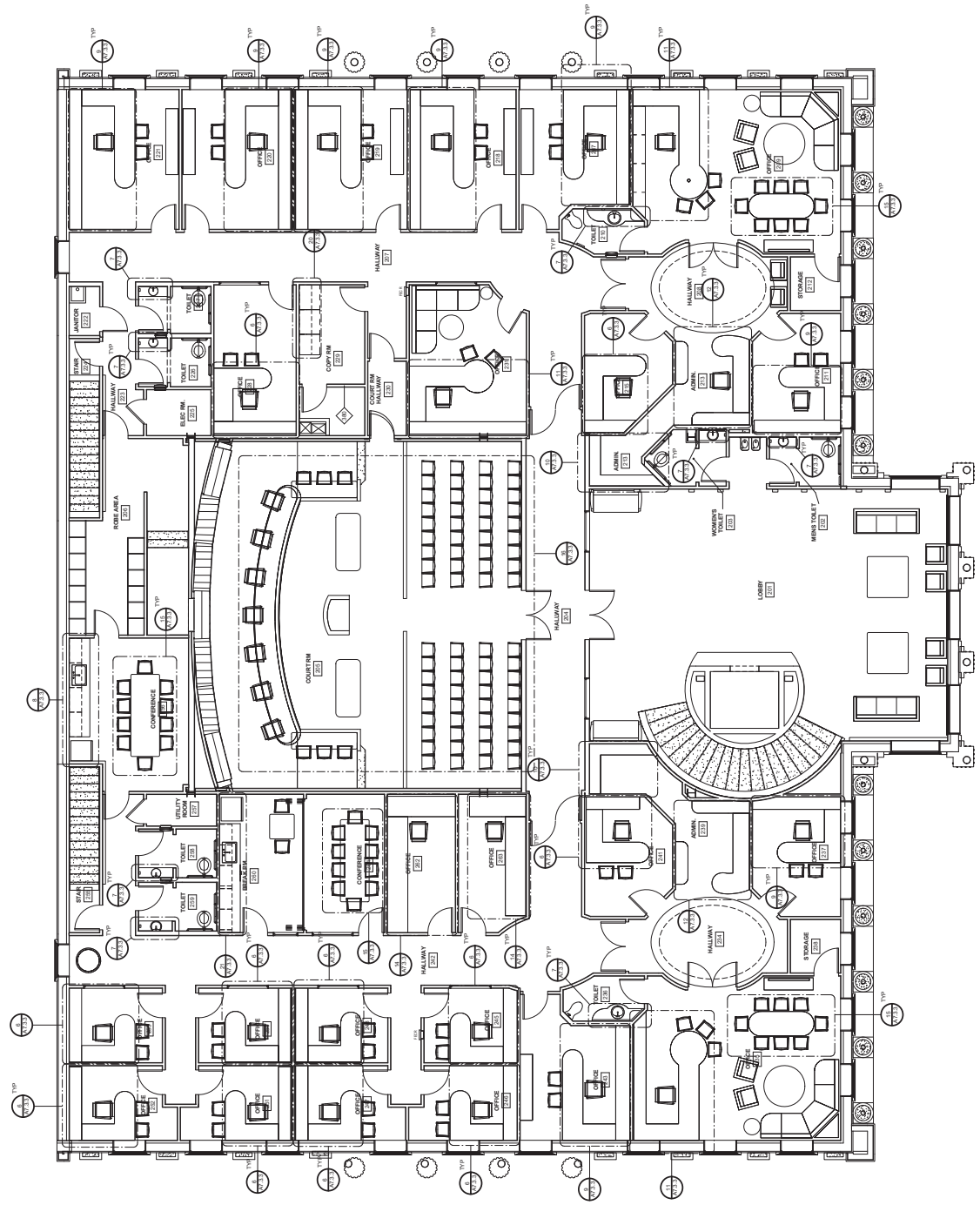
1 FLOOR PLAN - LEVEL 2 MILLWORK SCALE = 1/8\"/>
